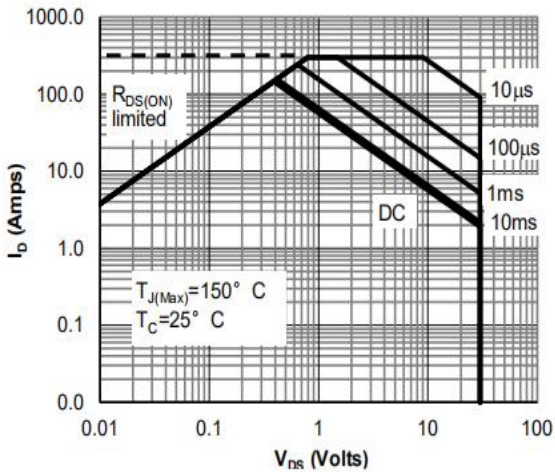
Figure 9: Maximum Forward Biased Safe Operating Area V GS > or equal to 4.5V
